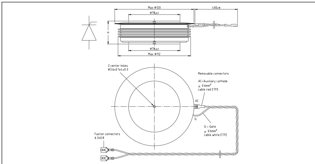
Fig. 18 Device Outline Drawing
